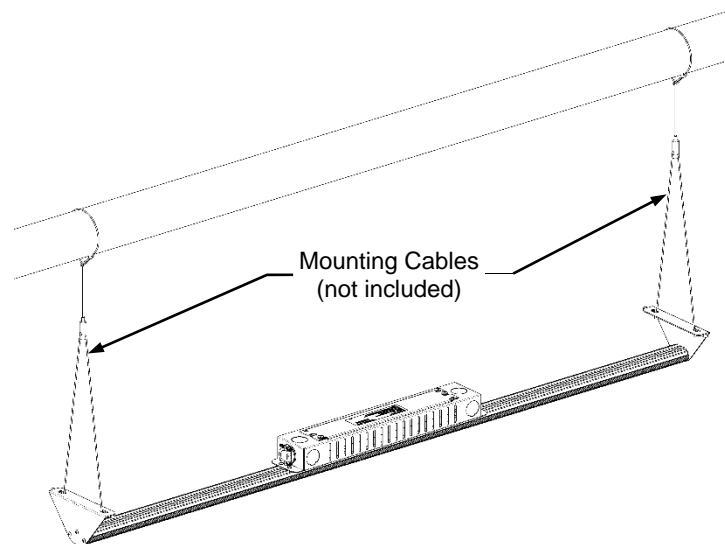
Figure 1a: Fixture Mounting (Suspended)
